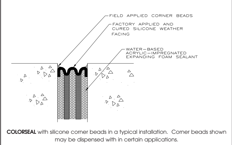
FIGURE 1: COLORSEAL in Typical Installation (substrates may vary).
