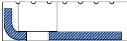
Premolded Steel Reinforced Elastomeric Anchor Block (P/N 2914)
