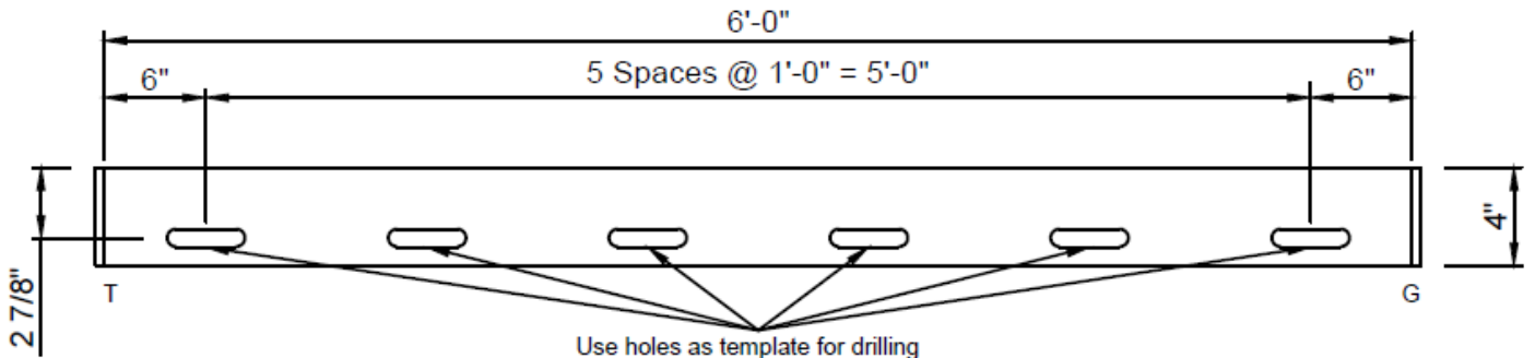
Plan View Standard Elastoflex Anchor Block
