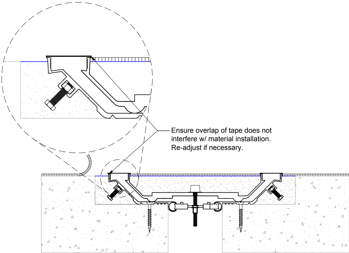
Carpet Shown - Finish floor material not by Emseal.
