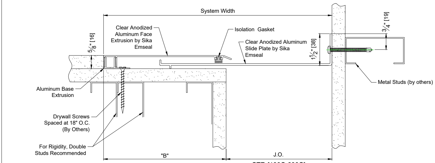
CTR-[100C-600C] WALL TO CORNER WALL CONDITION
