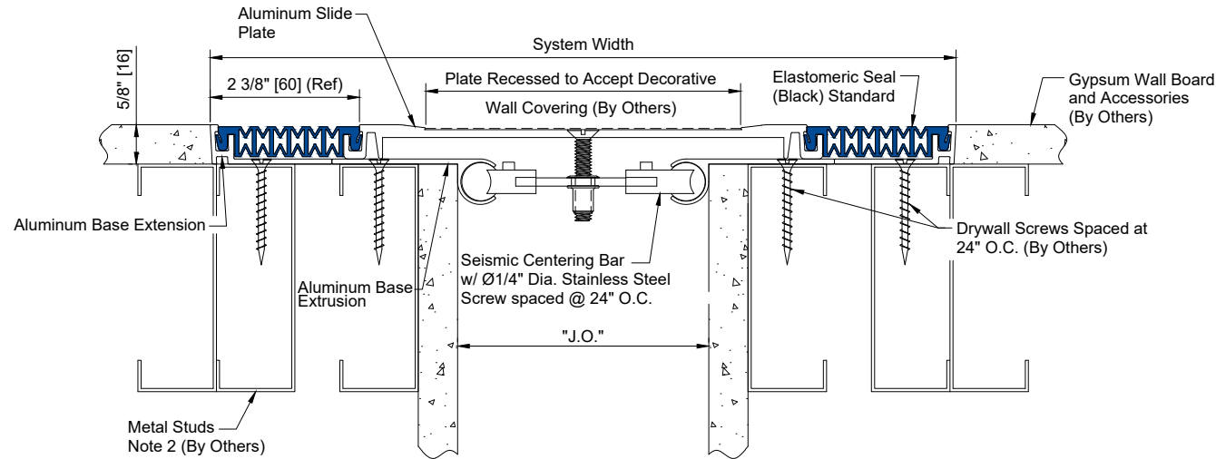
NBW [400-2400] WALL TO WALL CONDITION
