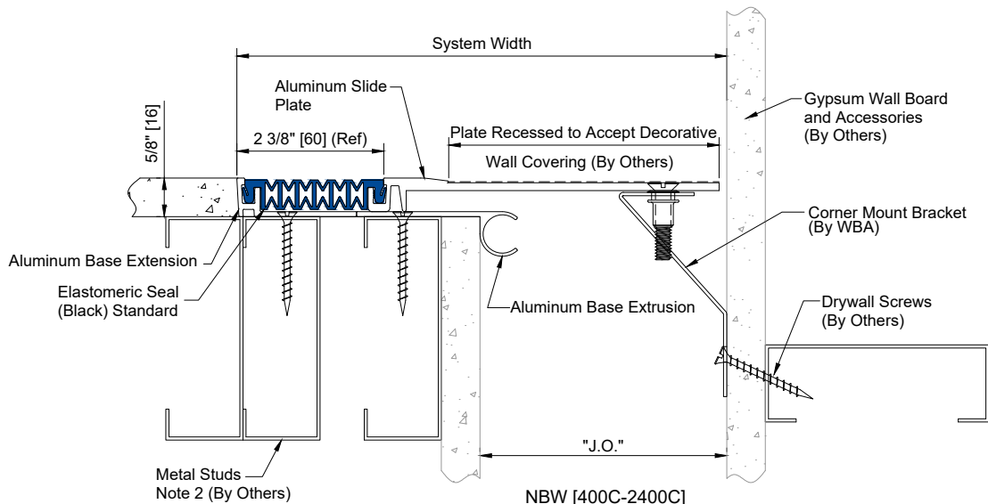
NBW [400C-2400C] WALL TO CORNER WALL CONDITION
